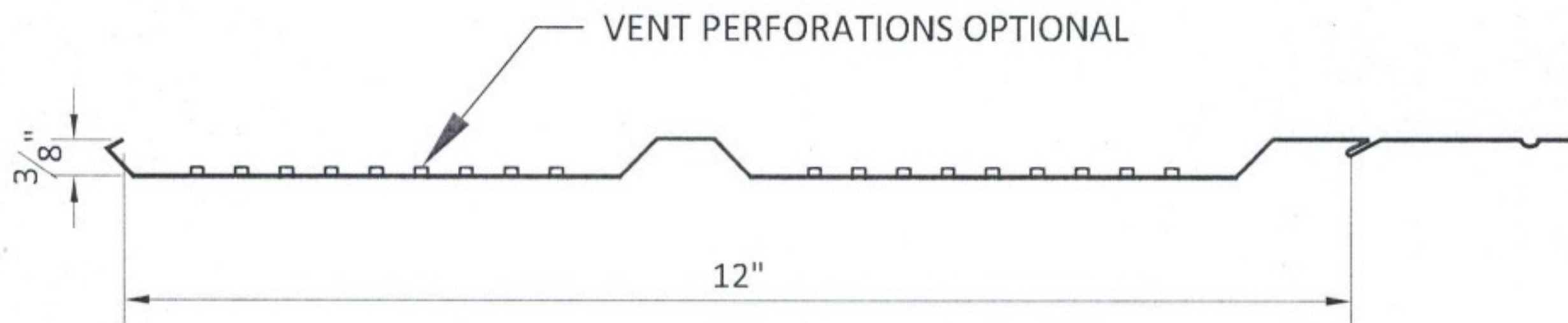
SOFFIT PANEL PROFILE
